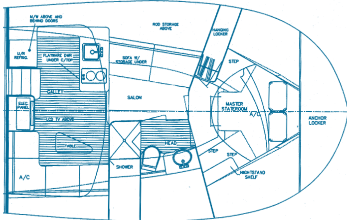
A- 45 Express Deck Plan B- 45 Express One-Stateroom Layout C- 45 Express Two-Stateroom Layout
