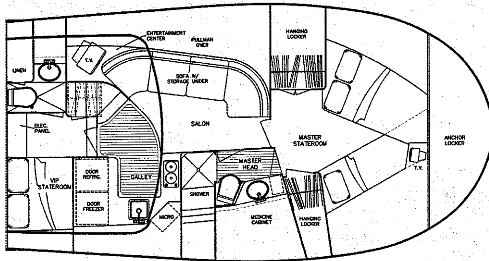
Interior Floor Plan "B" ▼
