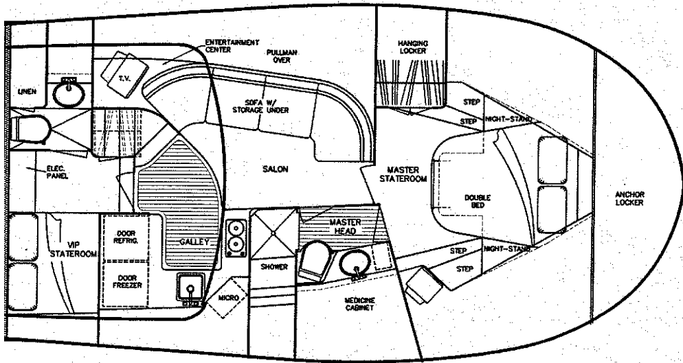
Interior Floor Plan "A" ▼
